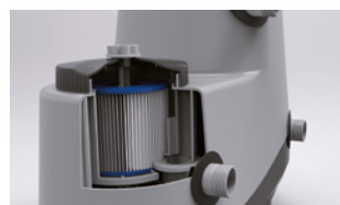
Filtration cartridge built into the pump
